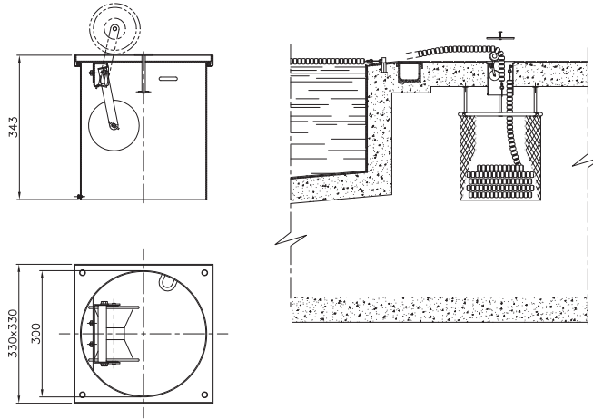
Fin type assembly diagram 1
